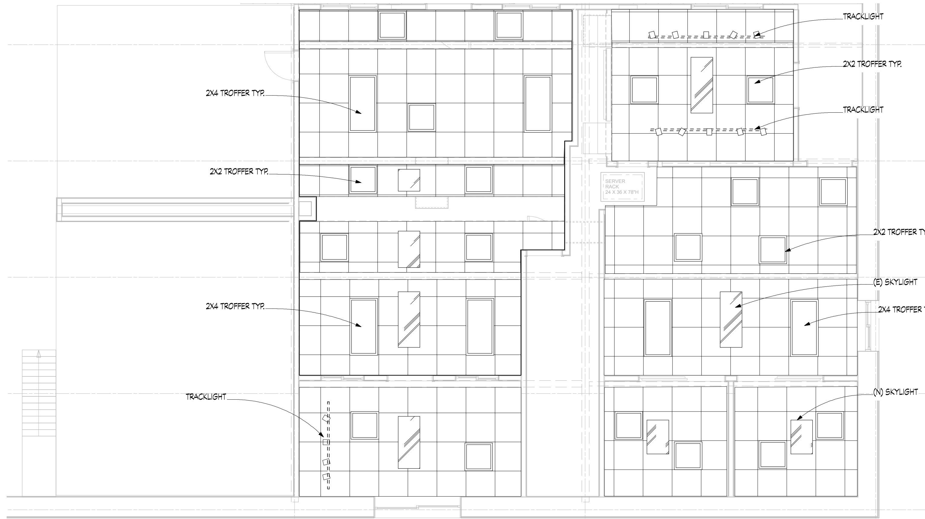
2 MEZZANINE LEVEL PROPOSED: RCP & LIGHTING 2.1 Scale: 1/4" = 1'-0"
