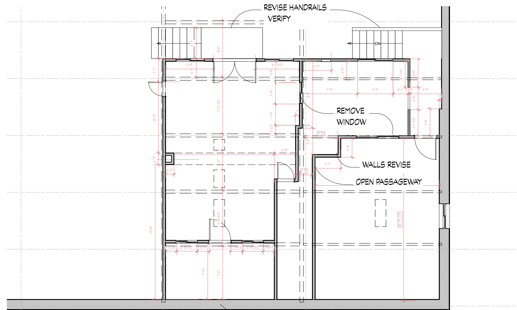
3 UPPER LEVEL EXISTING, DEMOLITION PLAN 2.1 Scale: 1/8" = 1'-0"
