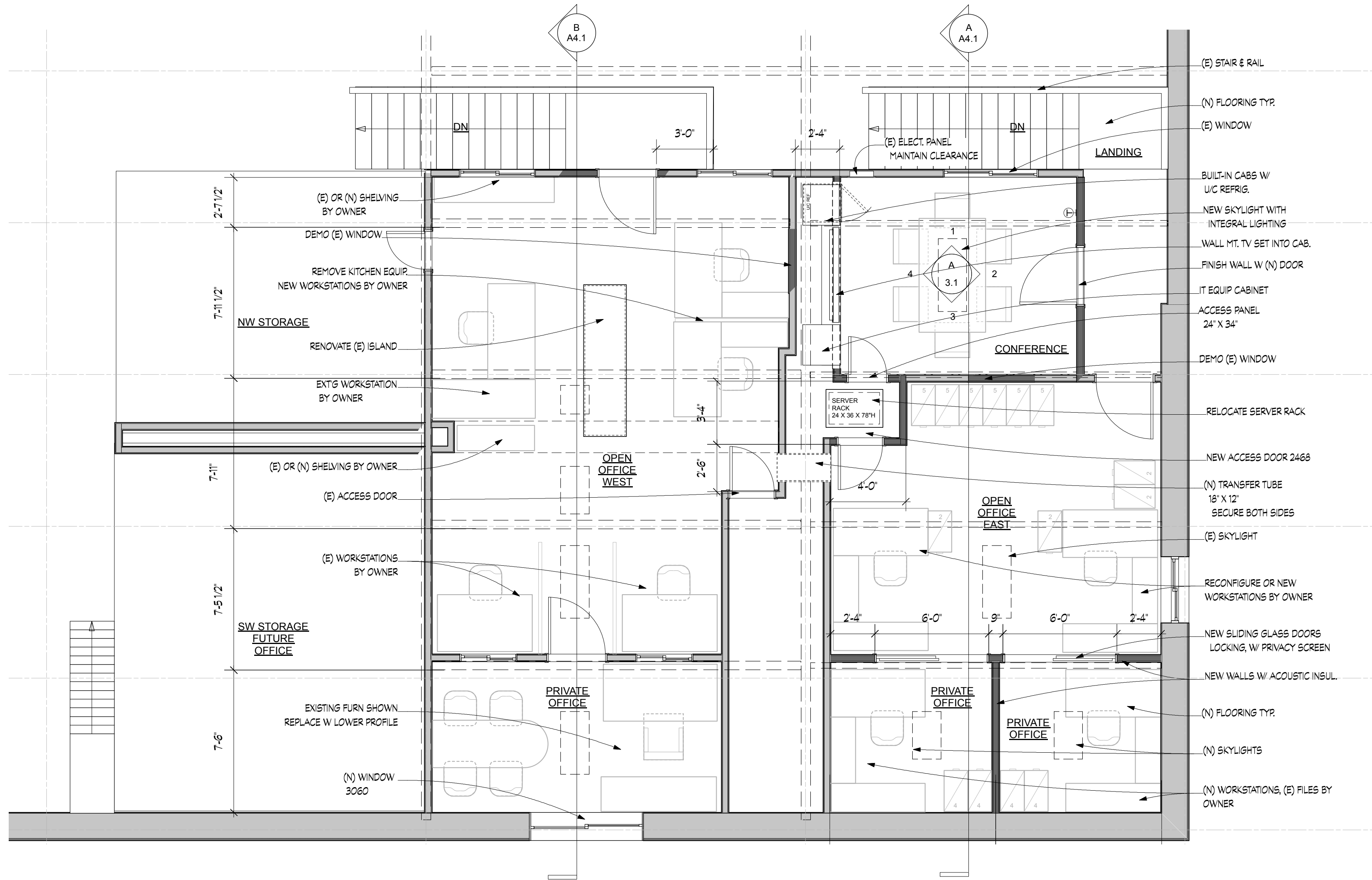
1 MEZZANINE LEVEL PROPOSED: CONSTRUCTION FLOOR PLAN 2.1 Scale: 1/4" = 1'-0"
